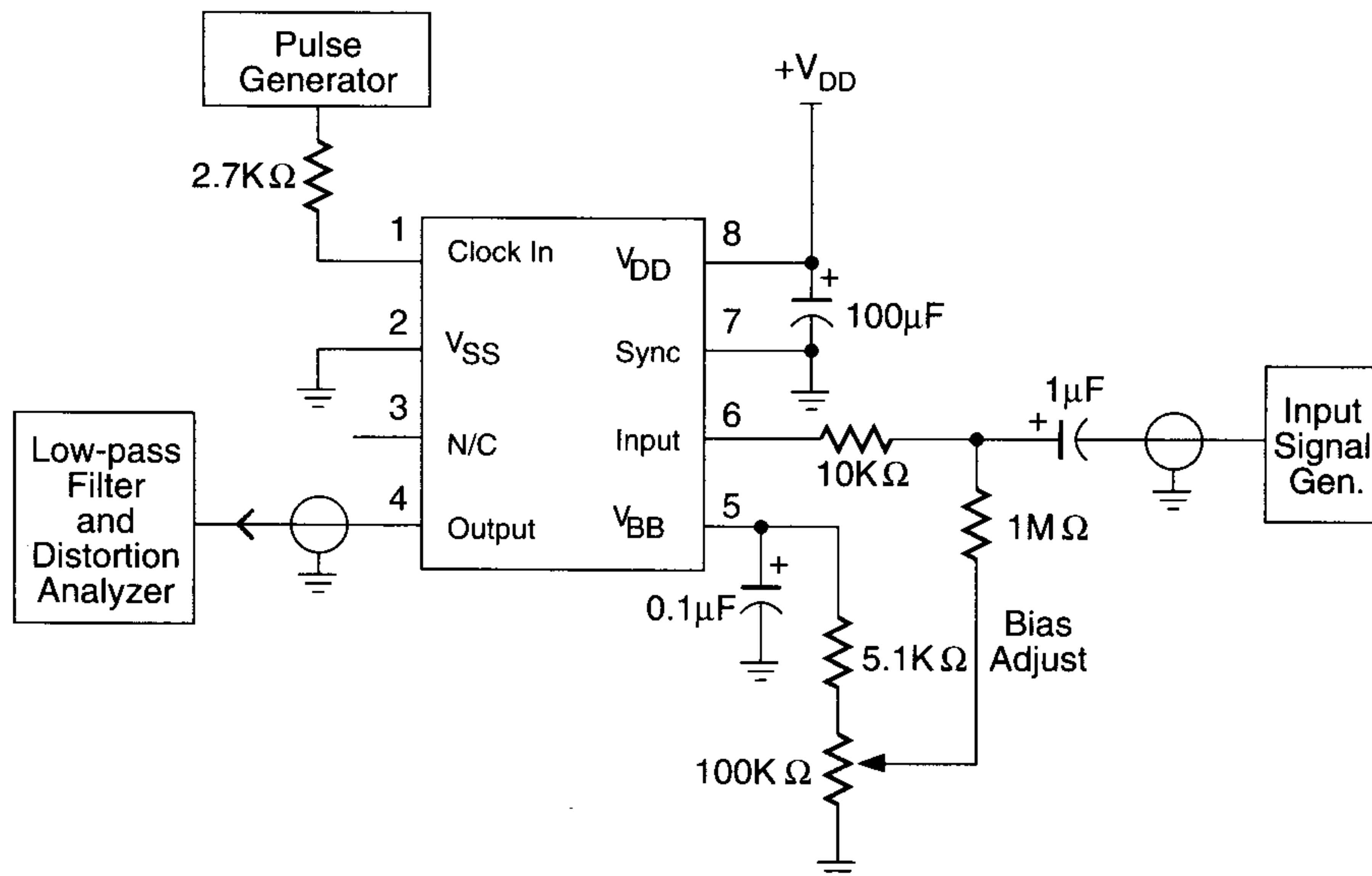
Figure 3. A Test Configuration
