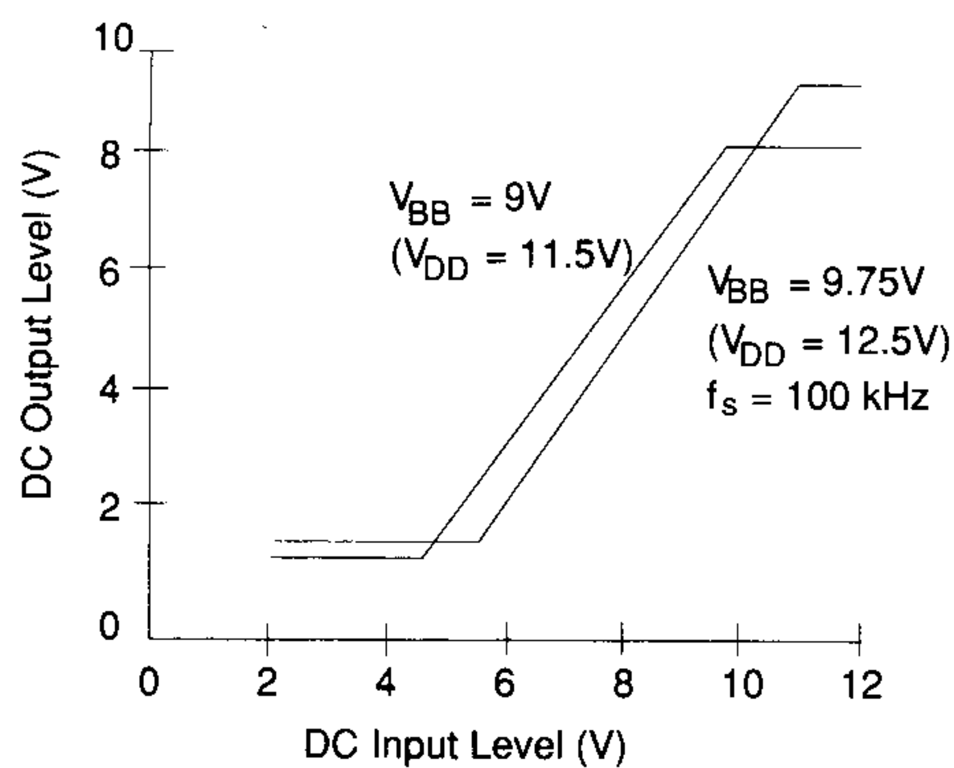
Figure 5. Typical DC Output vs. DC Input
