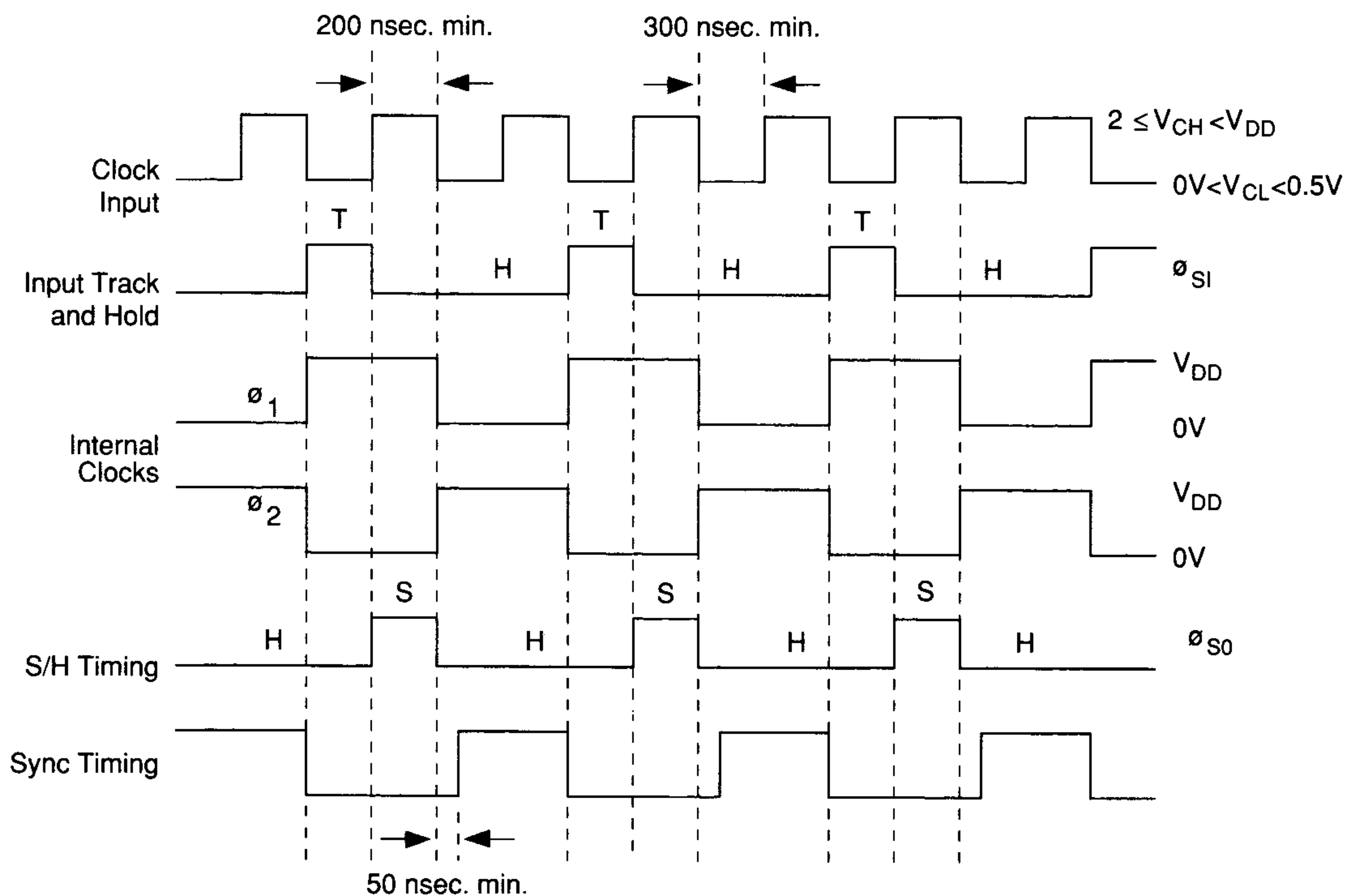
Figure 4. Timing Relations
