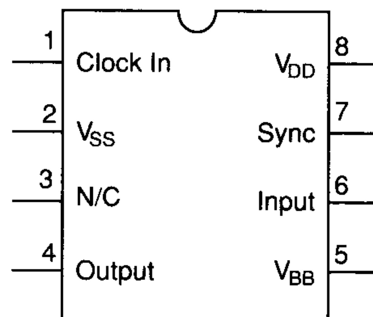
Figure 1. Pinout Configuration
