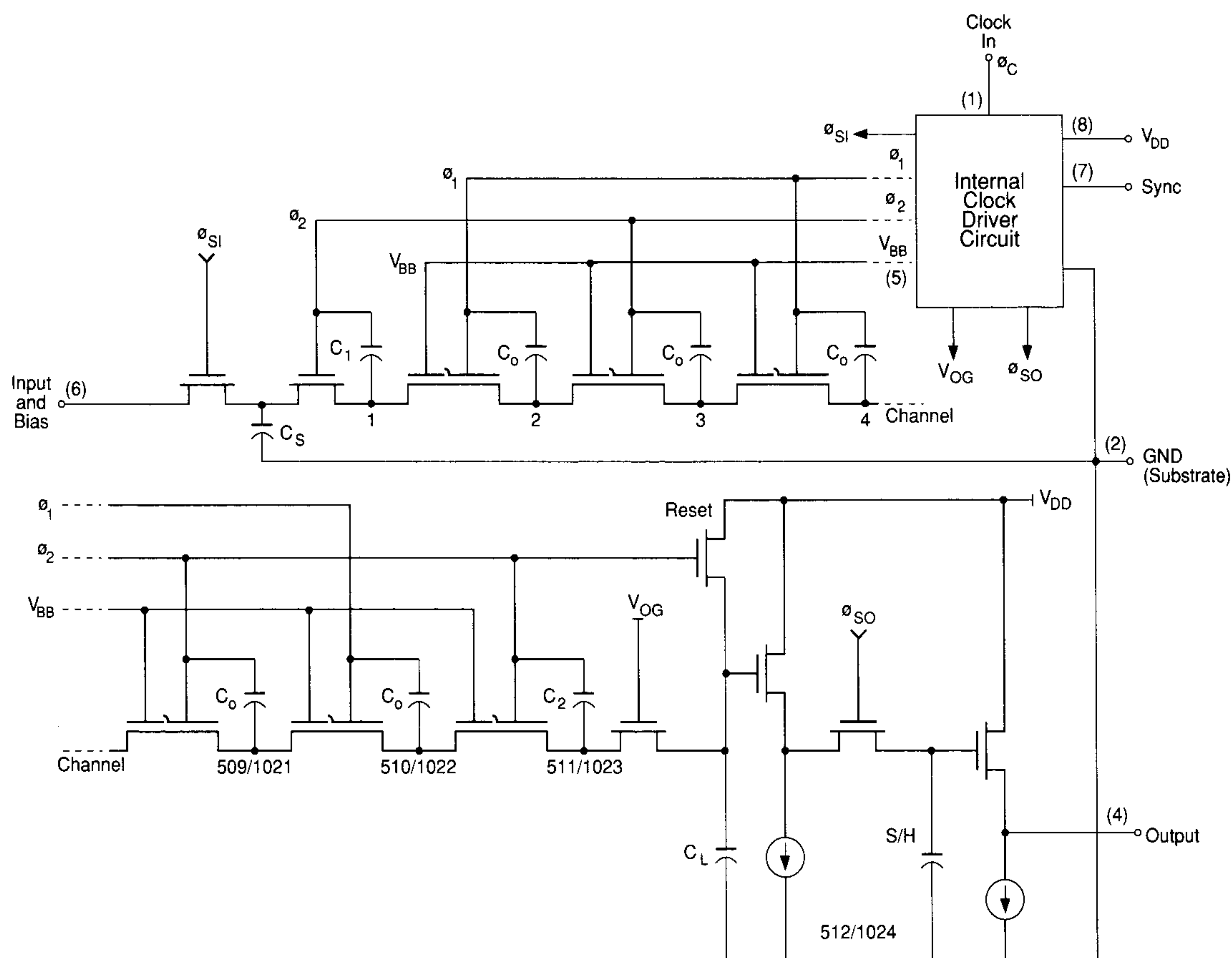
Figure 2. Equivalent Circuit
