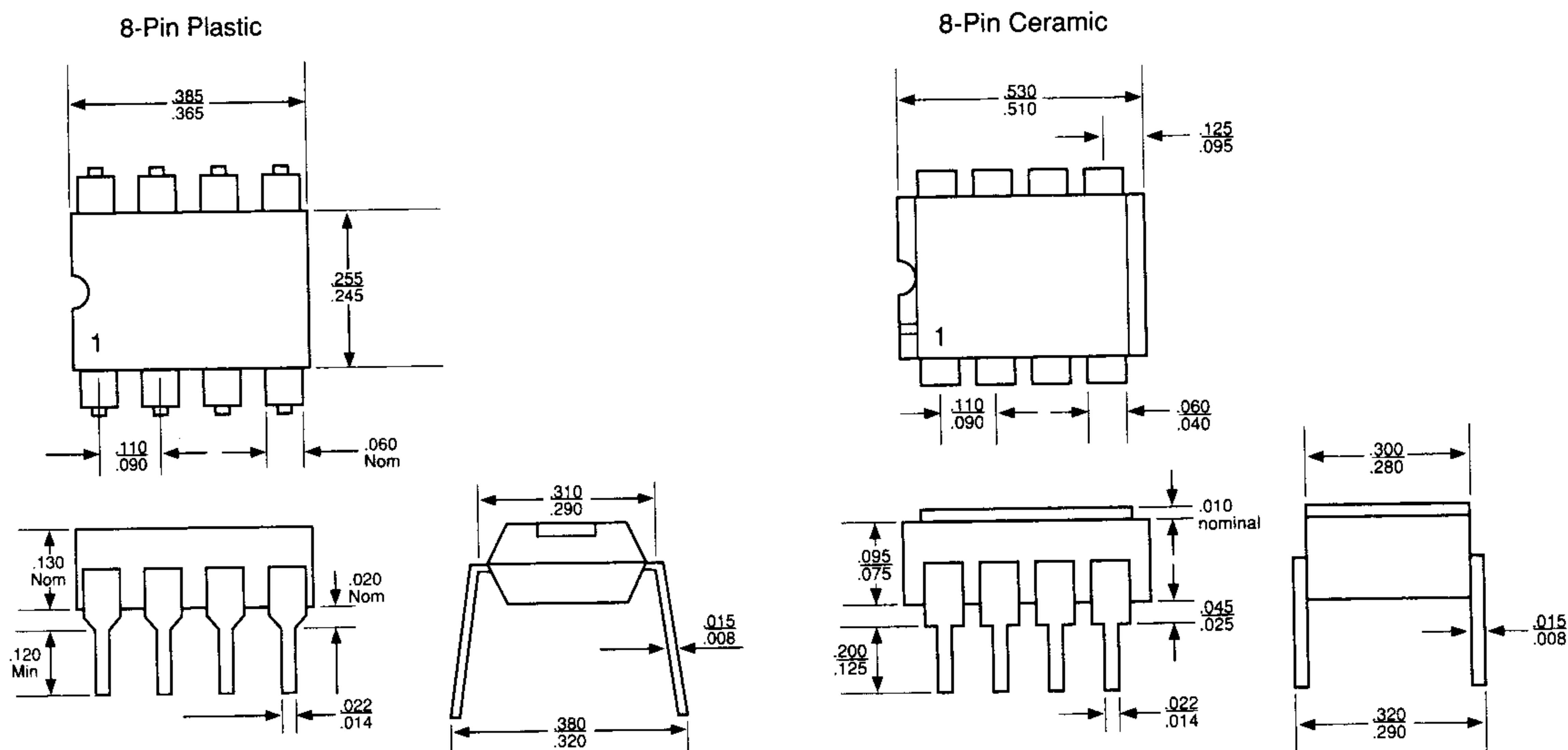
Figure 9. Package Dimensions
